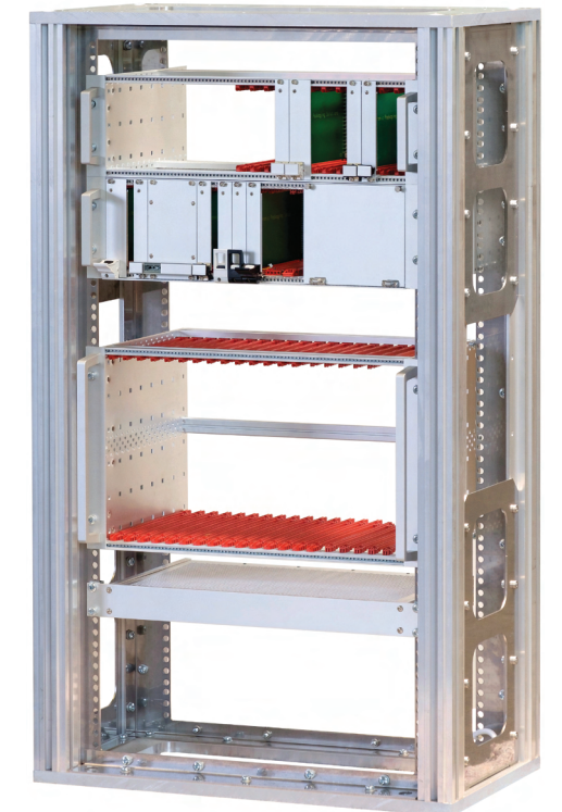
Vehicle OBR with a bolted aluminum frame
